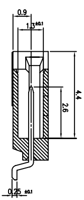
SEC A - A"
