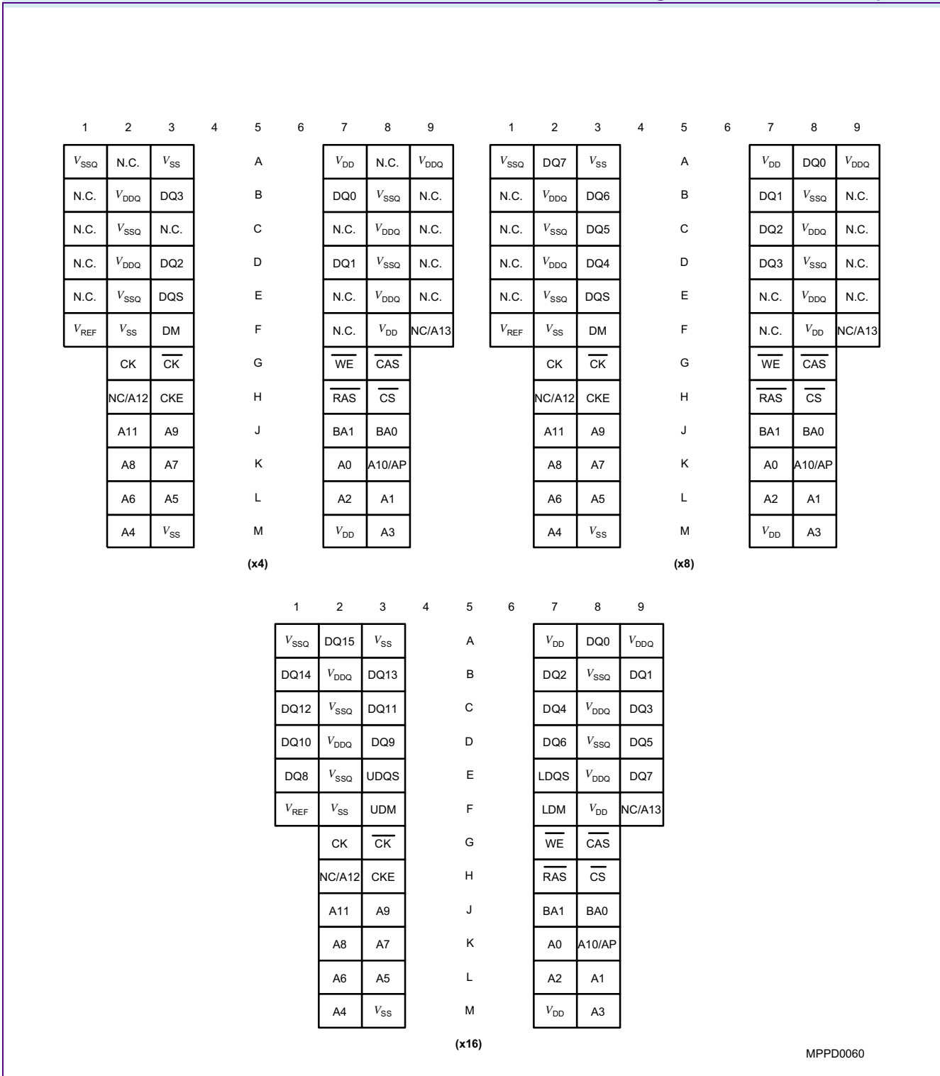
FIGURE 1 Pin Configuration P-TFBGA-60 Top View
